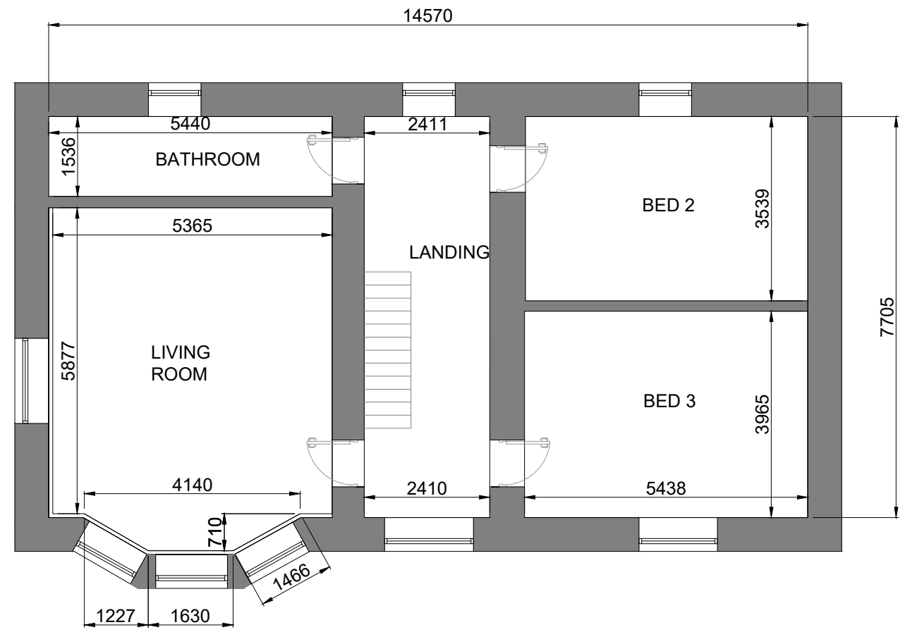
FIRST FLOOR
