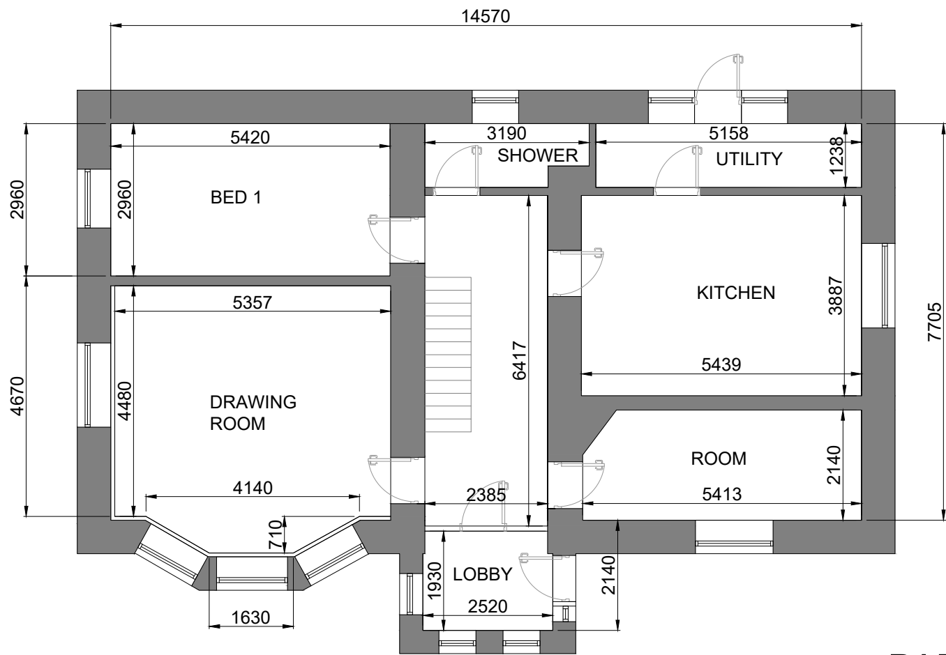
GROUND FLOOR
